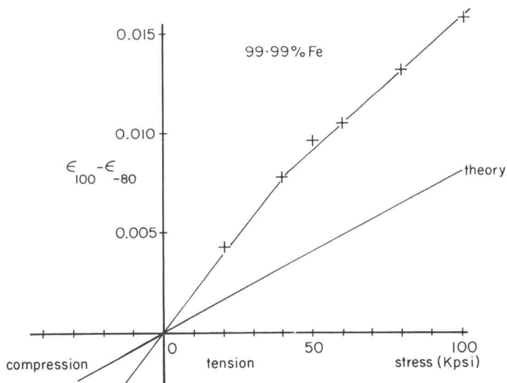
Figure 14. Relative count rates vs stress, ferrite.
